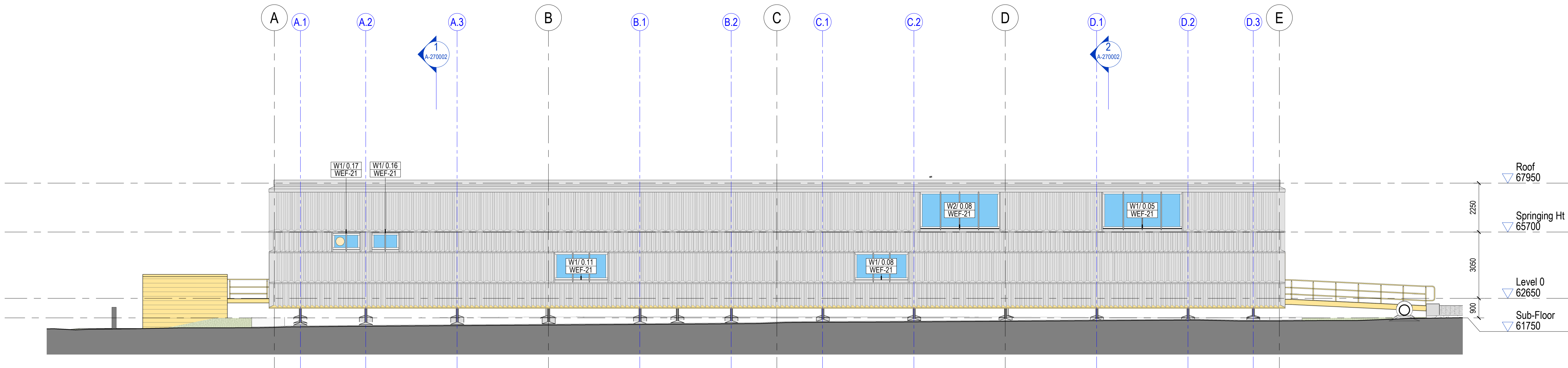
2 South Elevation 1 : 100
